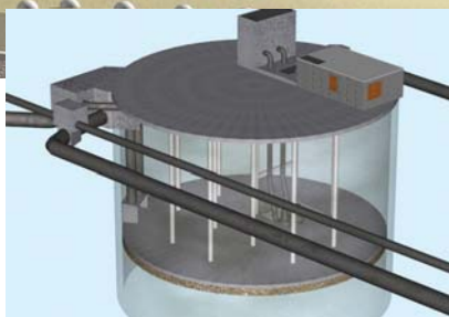
FRANCE - Floirac Storm tank
