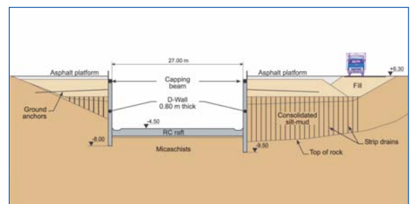
FRANCE - Concarneau Dry dock
